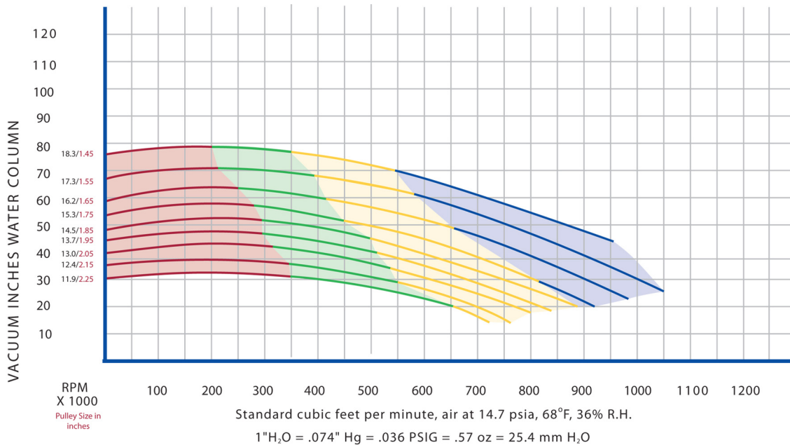
Vacuum vs. CFM
