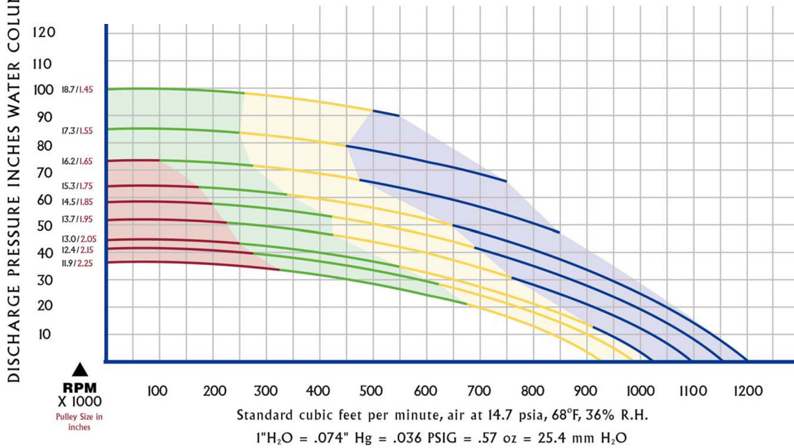
Pressure vs. CFM
