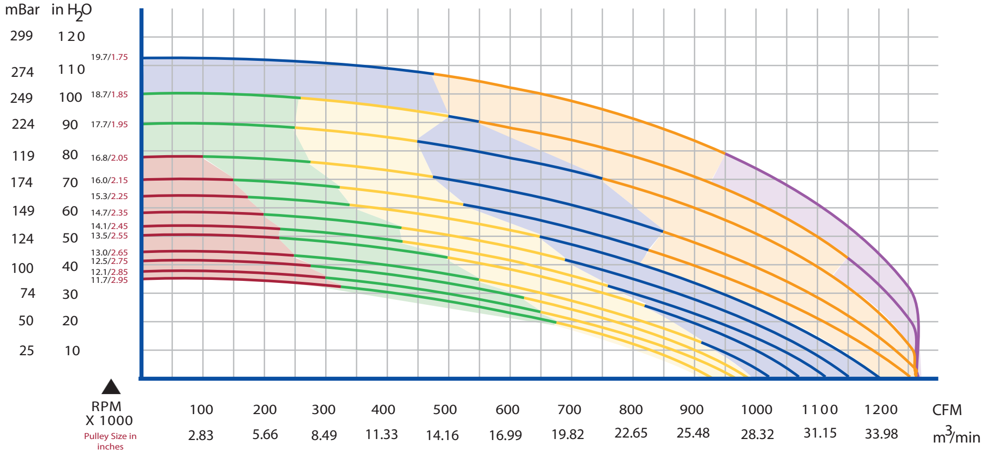
Pressure vs. CFM
