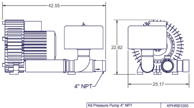
KPHRB1200 - Pressure Kit Drawing
