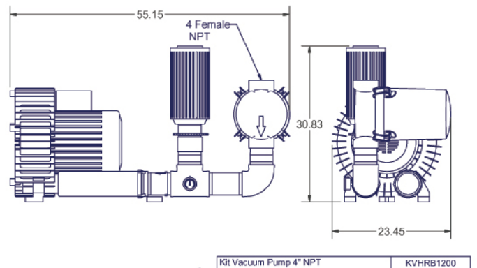
KVHRB1200 - Vacuum Kit Drawing
