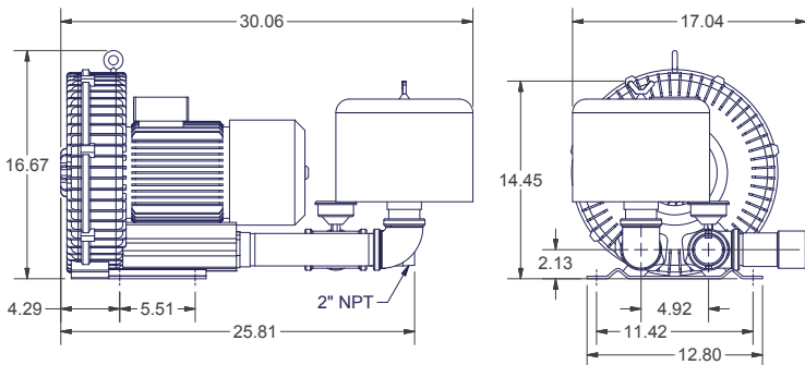
KPHRB700 - Pressure Kit Drawing
