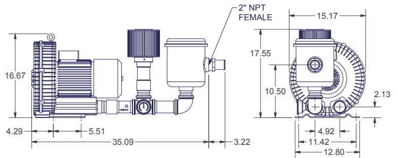
KVHRB700 - Vacuum Kit Drawing
